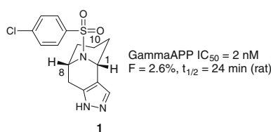
Figure 1. Representative N -bicyclic sulfonamide \gamma -secretase inhibitor.
