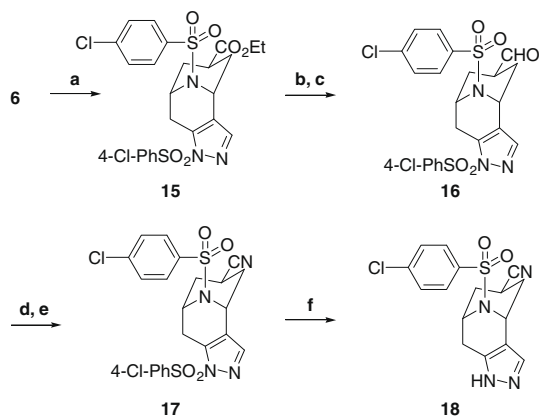
Scheme 3. Reagents and conditions: (a) 4-chlorobenzenesulfonyl chloride, pyridine, rt, 1 h, quant.; (b) LiBH 4 , THF, rt, 2 h, 86%; (c) Dess–Martin periodinane, NaHCO 3 , CH 2 Cl 2 , rt, 2 h, 87%; (d) NH 2 OH·HCl, pyridine/EtOH, rt, 2 h; (e) MsCl, Et 3 N, CH 2 Cl 2 , rt, 0.5 h; (f) NaOH, THF/H 2 O, rt, 5 h.
