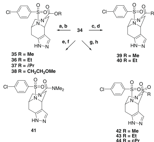
Scheme 8. Reagents and conditions: (a) ROC(O)Cl , Et_3N , CH_2Cl_2 , rt, 2 h; (b) NaOH, THF/ H_2O , 3 h, 70 °C; (c) (RCO)_2O , pyridine, rt, 5 h; (d) NaOH, THF/ H_2O , 2 h, rt; (e) N,N -dimethylcarbamyl chloride, Et_3N , CH_2Cl_2 , 2 days, rt; (f) NaOH, THF/ H_2O , 40 h, 70 °C; (g) RSO_2Cl , Et_3N , CH_2Cl_2 , 1 h, rt; (h) NaOH, THF/ H_2O , 2 h, 60 °C.
