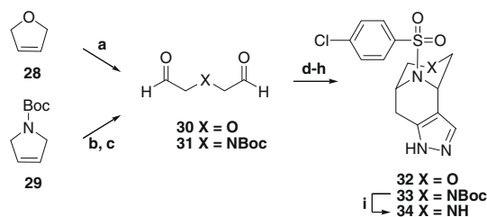
Scheme 7. Reagents and conditions: (a) O_3 , CH_2Cl_2/CH_3OH , 10/1, v/v, Ph_3P , rt, 2 h; (b) OsO_4 , NMO, acetone, rt, 18 h; (c) NaIO_4 , THF/ H_2O , rt, 3 h; (d) acetone-1,3-dicarboxylic acid, BnNH_2 NaOAc HCl (aq), 3 days, rt; (e) Pearlman's catalyst, H_2 (30 psi), CH_3OH , 12 h, rt; (f) 4-chlorobenzenesulfonyl chloride, Et_3N , CH_2Cl_2 , 2 h, rt; (g) ethyl formate, NaOEt, THF/ EtOH , 0.5 h, 60 °C; (h) hydrazine monohydrate, AcOH, EtOH , 1 h, rt; (i) HCl/dioxane, 2 h, rt.
