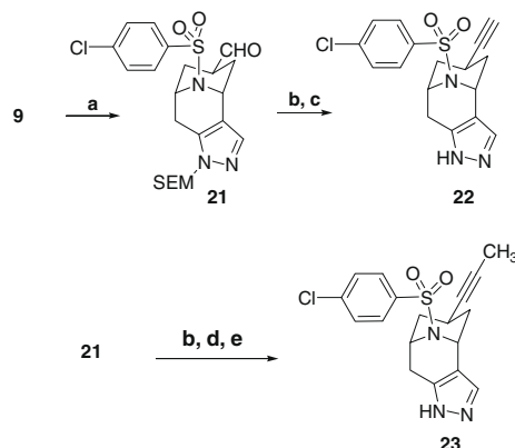
Scheme 5. Reagents and conditions: (a) oxalyl chloride, DMSO, Et 3 N, CH 2 Cl 2 , –78 °C to rt, 2 h, 64%; (b) Ohira–Bestmann reagent, K 2 CO 3 , CH 3 OH, rt, 18 h 70%; (c) HCl, dioxane/CH 3 OH, 1 h, 60 °C, 90%; (d) LiHMDS, CH 3 I, THF, –78 °C to rt, 4 h, 95%; (e) HCl, dioxane/CH 3 OH, 4 h, 60 °C, quant.
