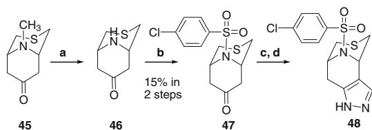
Scheme 9. Reagents and conditions: (a) ACE, \text{CH}_2\text{Cl}_2 , reflux, 6 h; (b) 4-chlorobenzenesulfonyl chloride, \text{Et}_3\text{N} , \text{CH}_2\text{Cl}_2 , 2 h, rt, 15% (2 steps); (c) ethyl formate, \text{NaOEt} , \text{THF/EtOH} , 0.5 h, 60^\circ\text{C} ; (d) hydrazine monohydrate, \text{AcOH} , \text{EtOH} , 1 h, rt, 25% (2 steps).
