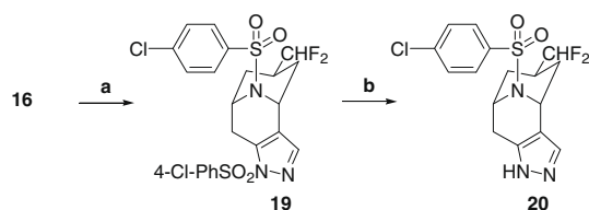
Scheme 4. Reagents and conditions: (a) DAST, CH 2 Cl 2 , 0 °C, 1 h; (b) NaOH, THF/H 2 O, 60 °C, 3 h 31% (2 steps).
